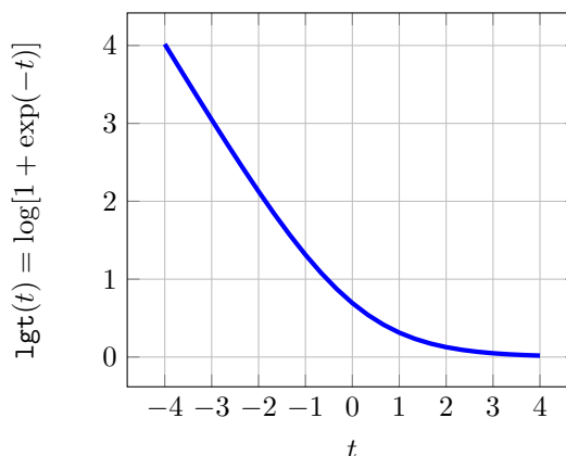
logistic loss
